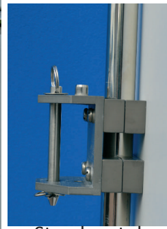
Stand up tube secured by clamp blocks
